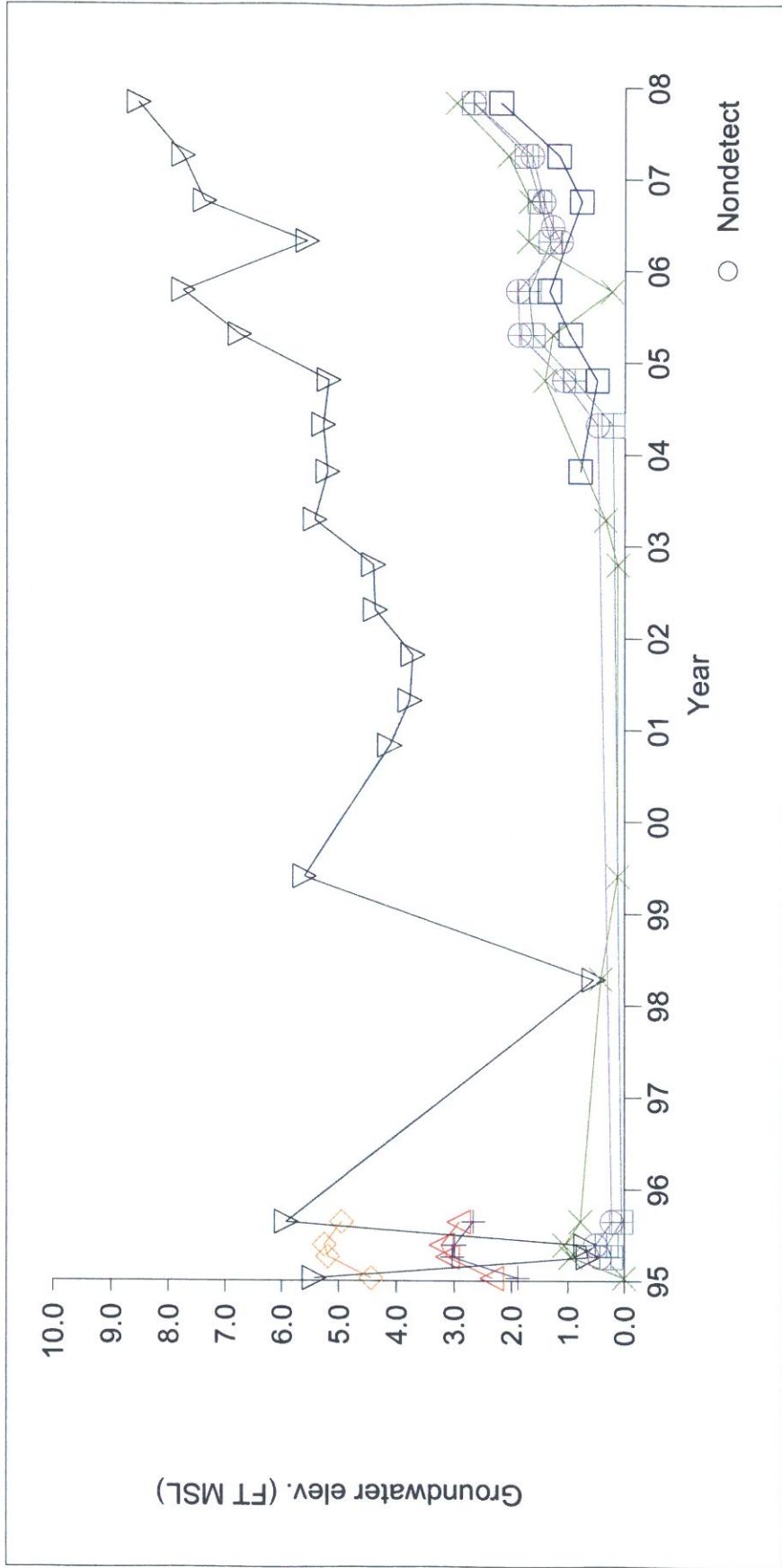
Chicot Aquifer - Unit IV Time Series Plot for Groundwater Elevation
