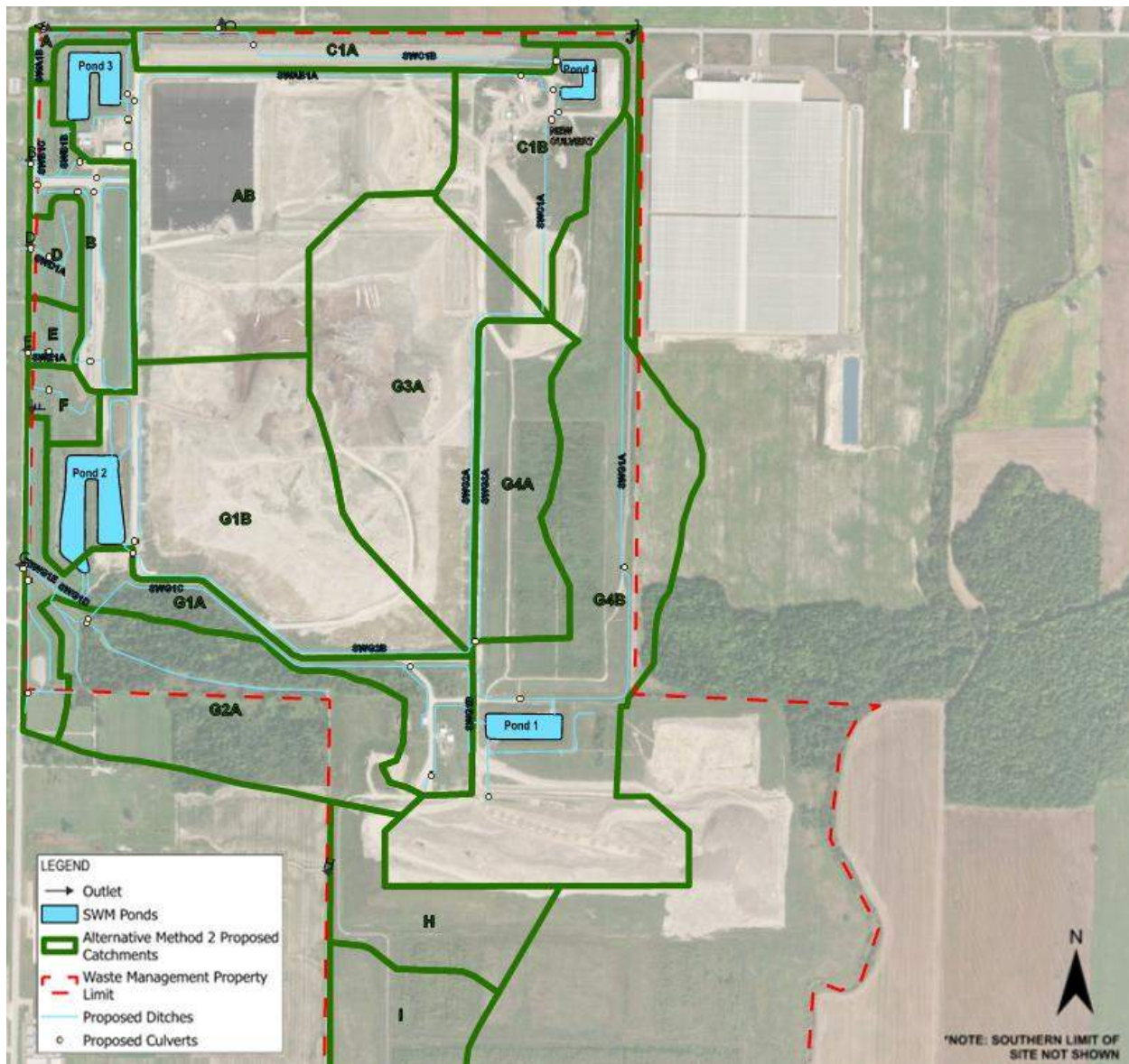
Figure 4-1. Stormwater Management for Alternative Method 3
