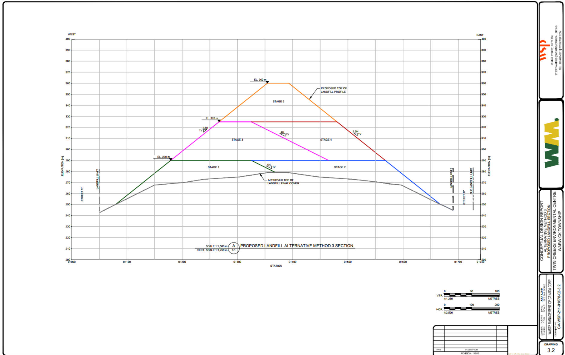
Figure 1-6. Alternative Method 3 – Landfill Section
