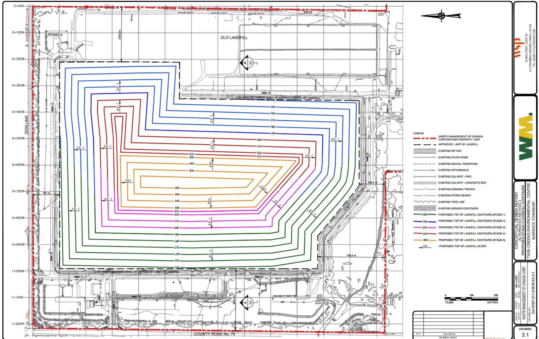
Figure 1-5. Alternative Method 3 – Landfill Contours
