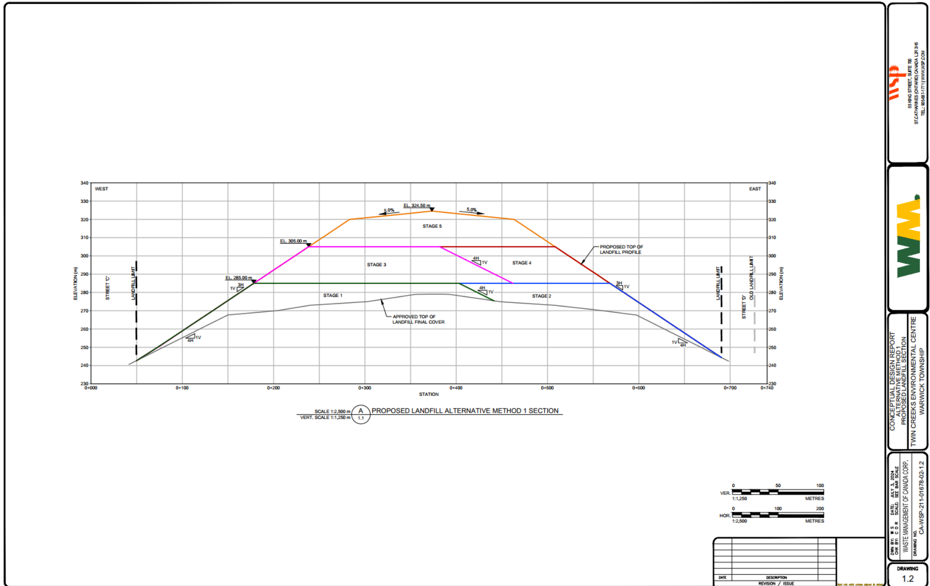
Figure 1-2. Alternative Method 1 – Landfill Section
