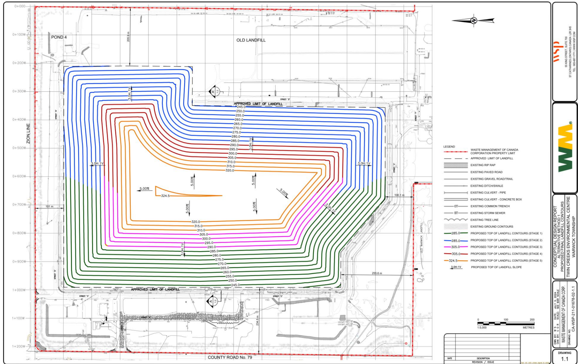
Figure 1-1. Alternative Method 1 – Landfill Contours
