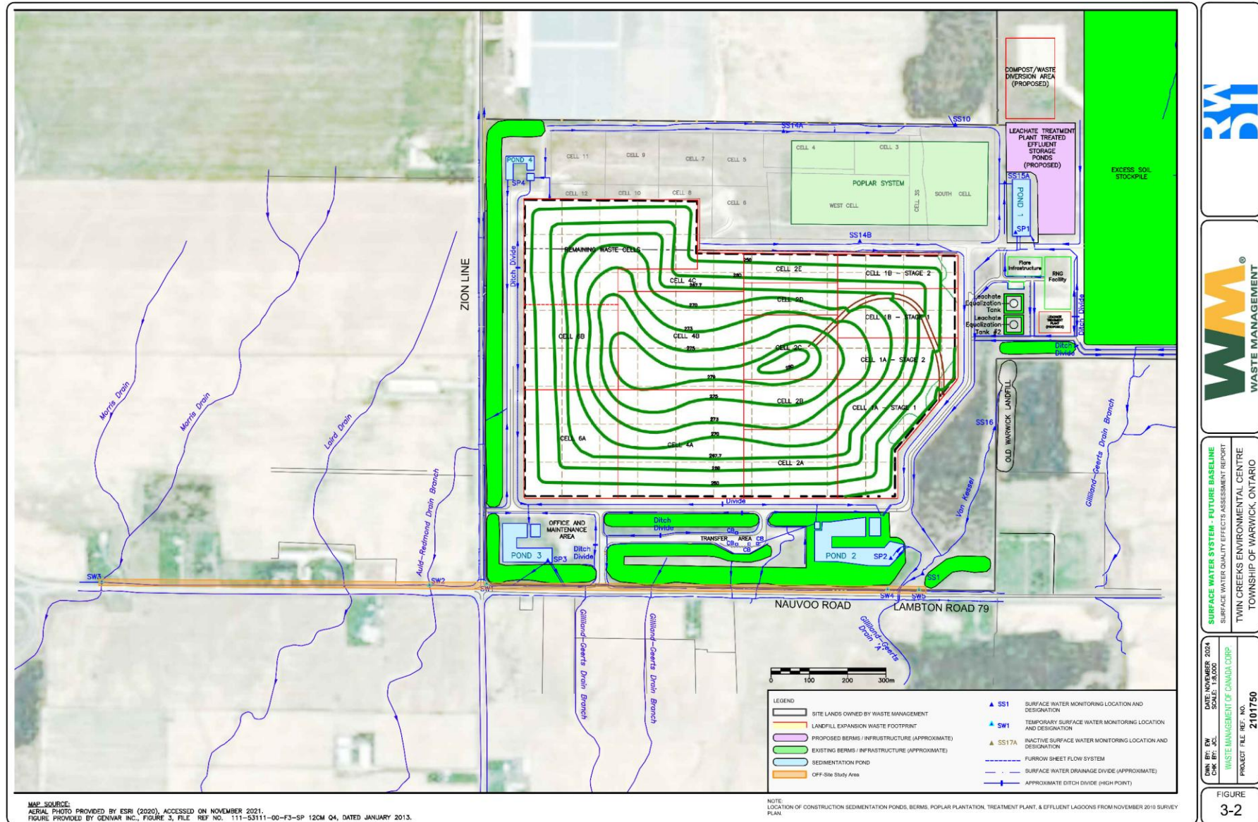
Figure 3-2. Off-Site Study Area – Future Baseline Conditions
