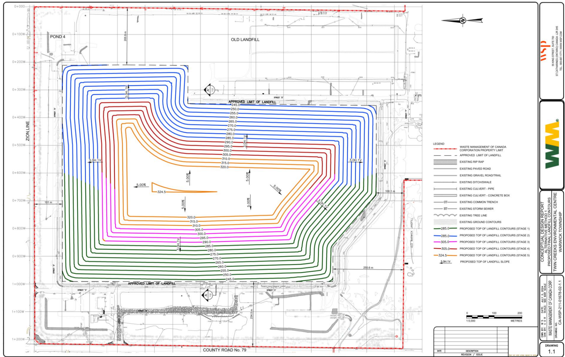
Figure 1-1. Alternative Method 1 Proposed Landfill Contours
