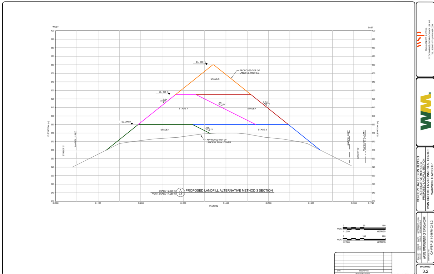
Figure 1-8. Alternative Method 3 Proposed Landfill Cross-section
