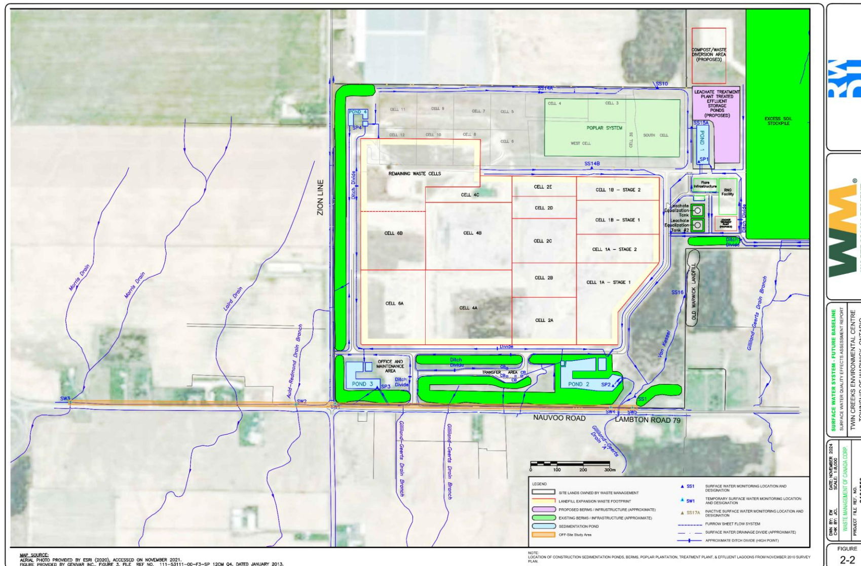
Figure 2-2. Off-Site Study Area (Showing the Surface Water Drainage Network as well as On-Site and Off-Site Surface Water Monitoring Stations)
