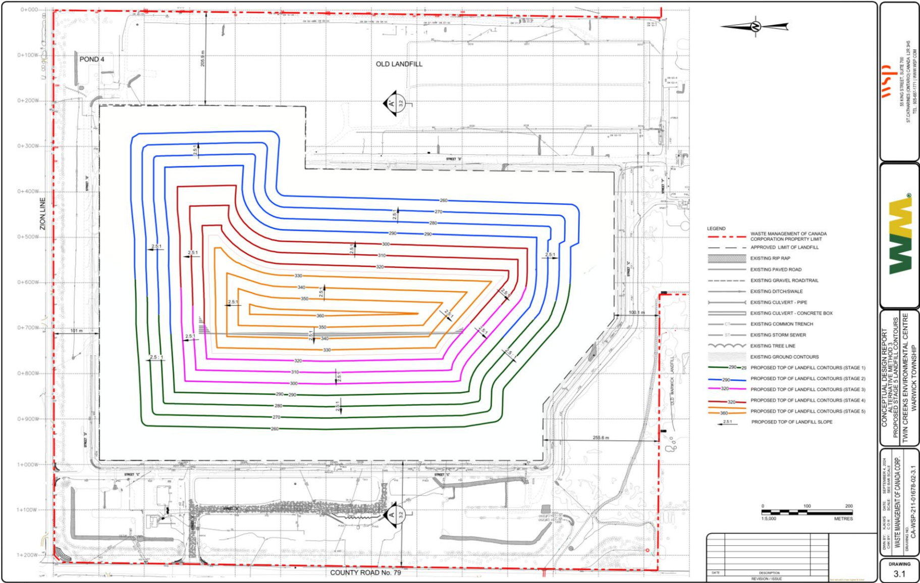
Figure 1-7. Alternative Method 3 Proposed Landfill Contours
