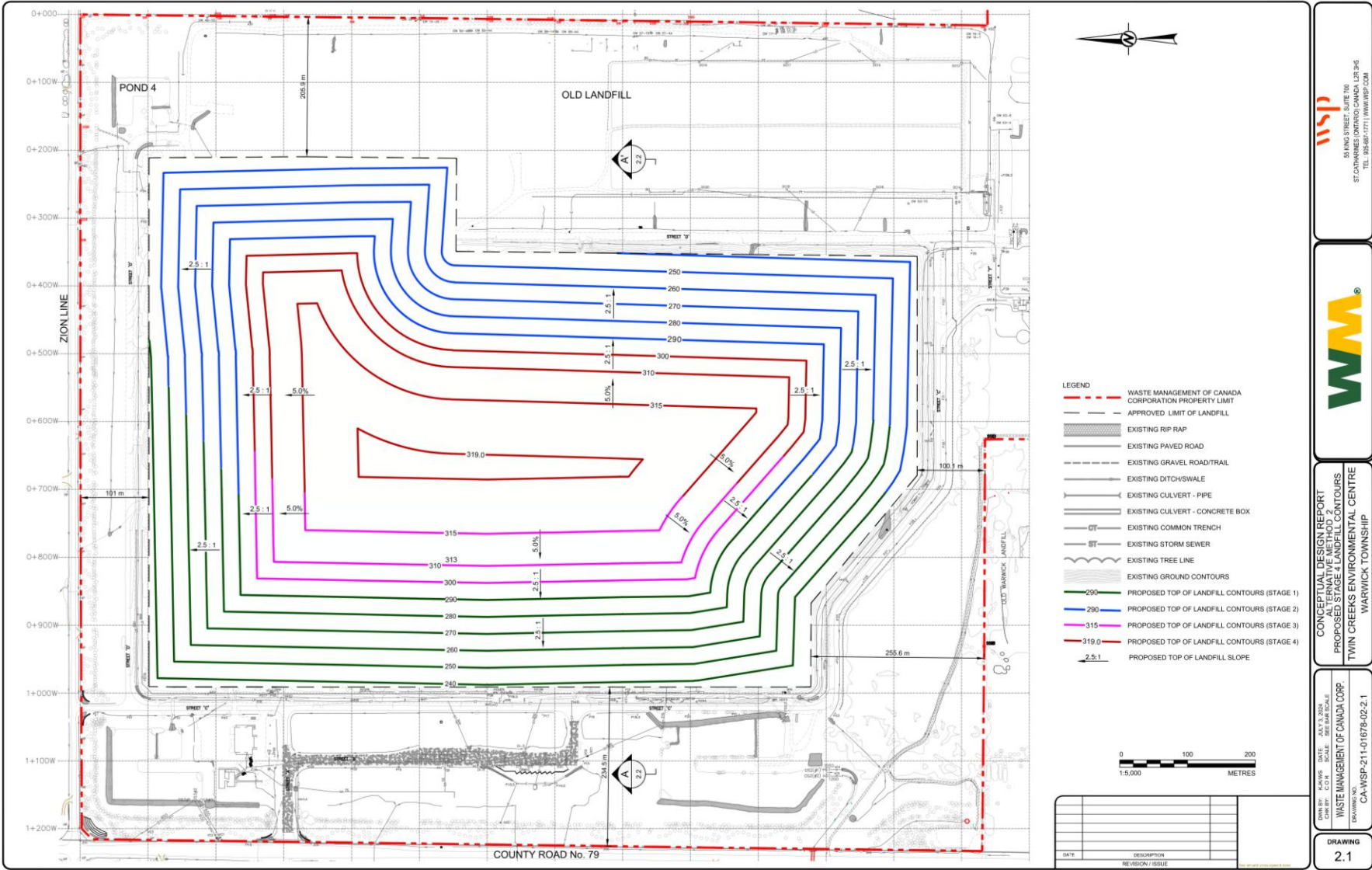
Figure 1-4. Alternative Method 2 Proposed Landfill Contours
