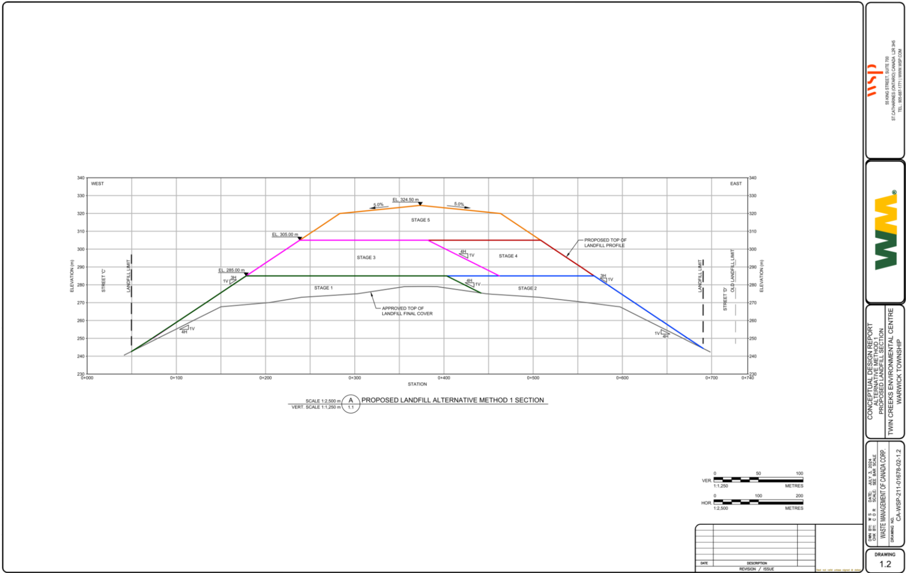
Figure 1-2. Alternative Method 1 Proposed Landfill Cross-section
