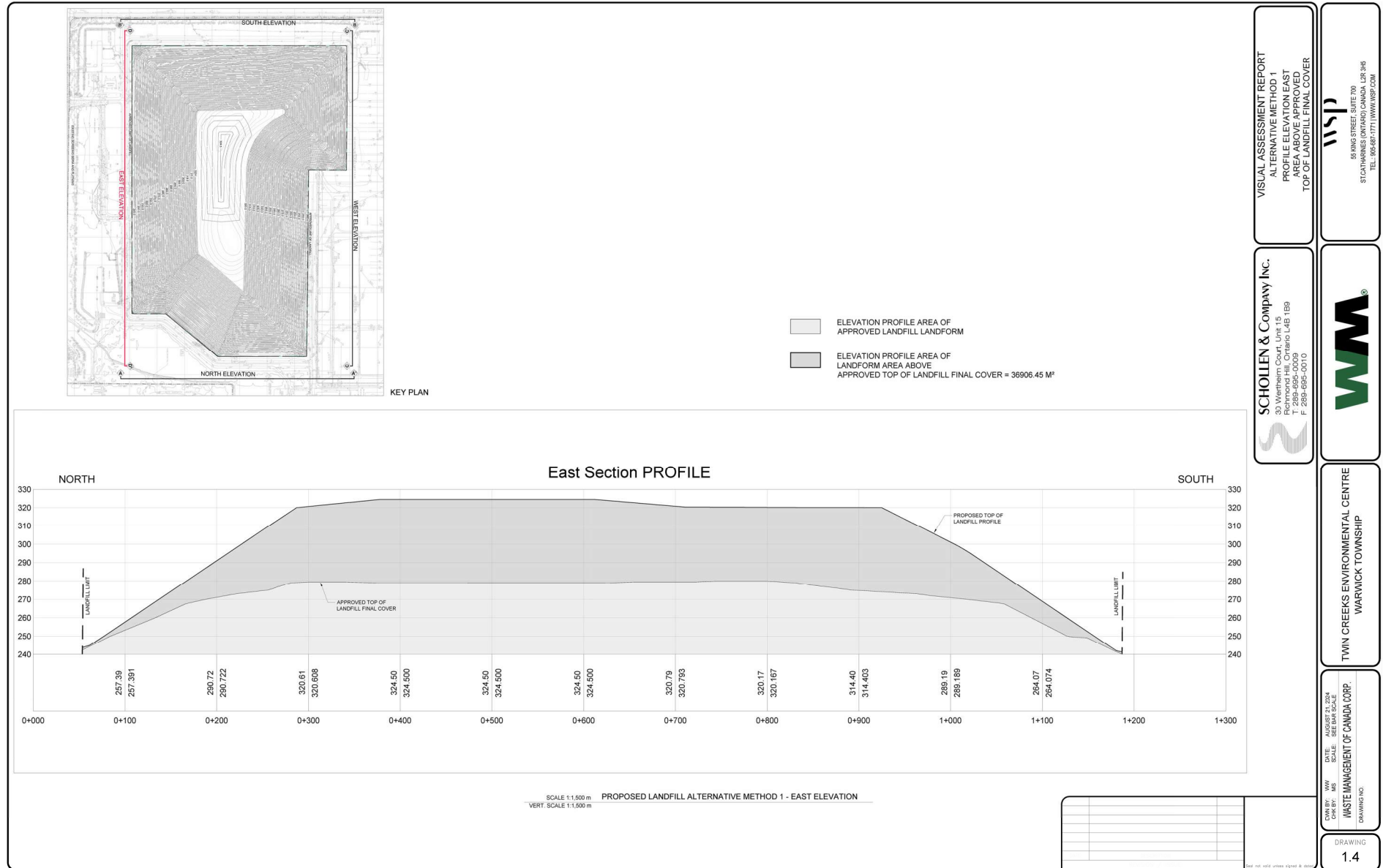
Figure 1-4. Alternate Method 1 – Profile Elevation East – Area Above Approved Top of Landfill Final Cover
