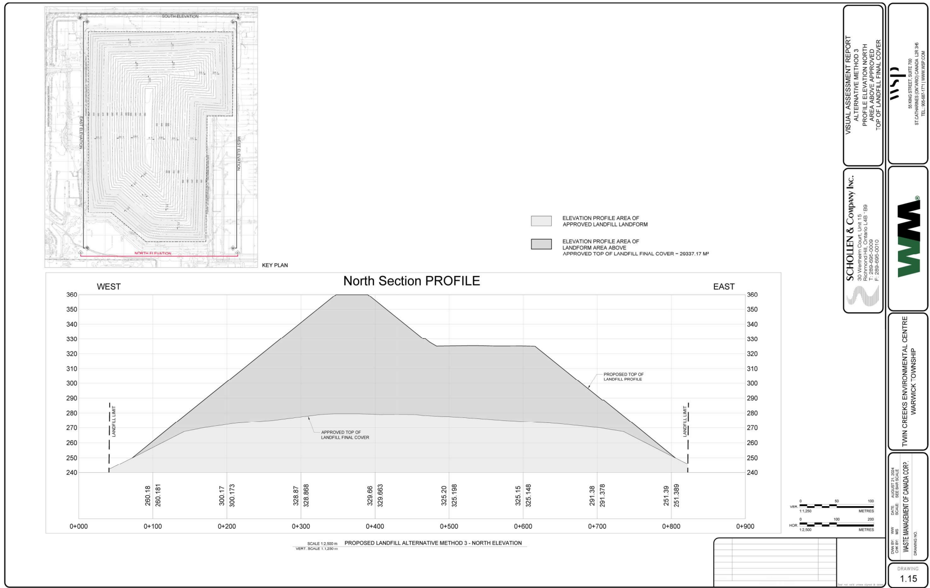
Figure 1-15. Alternate Method 3 – Profile Elevation North – Area Above Approved Top of Landfill Final Cover
