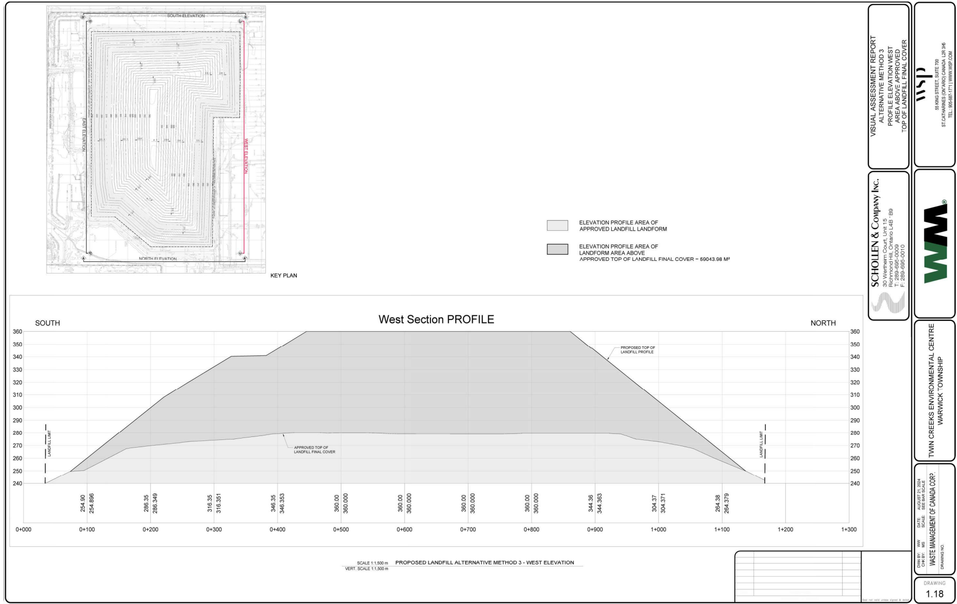
Figure 1-18. Alternate Method 3 – Profile Elevation West – Area Above Approved Top of Landfill Final Cover
