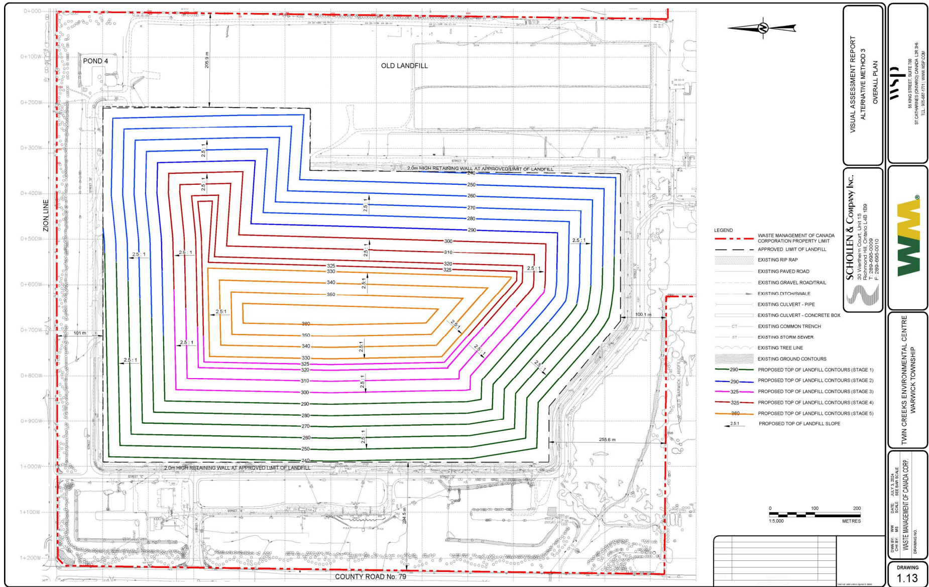
Figure 1-13. Alternate Method 3 – Overall Plan
