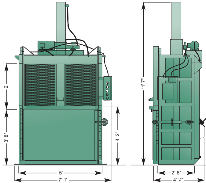
Vertical Baler
