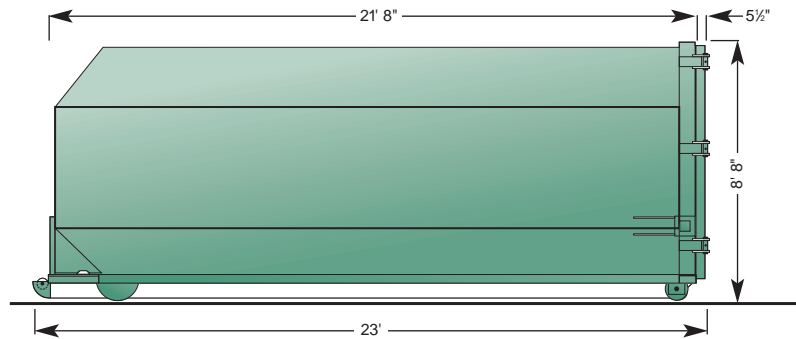
40-Yard Receiving Container
