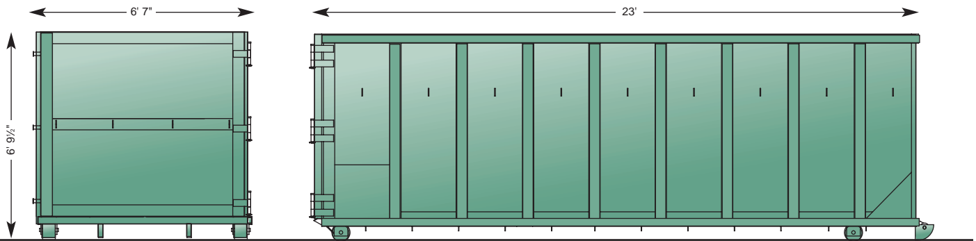
40-Yard Open-Top Container
