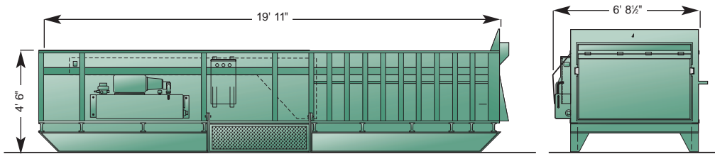
5-Yard Stationary Compactor
