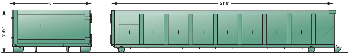
20-Yard Open-Top Container
