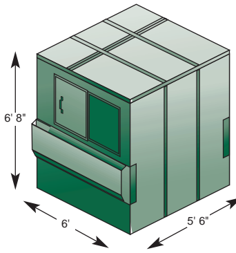
8-Yard Bin
