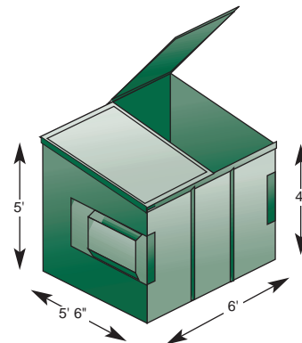
4-Yard Bin
